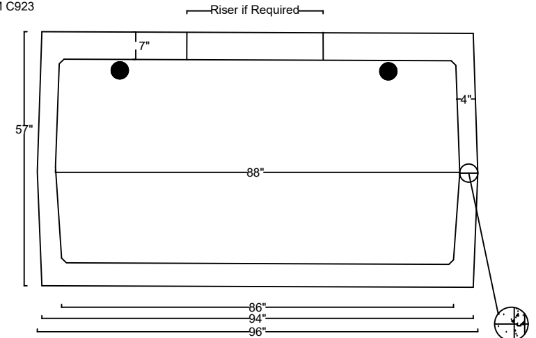
End View
